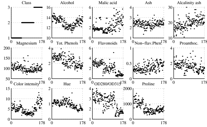
Fig. 3. Wine data: 3 classes and 13 attributes.
