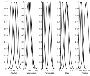
Fig. 5. Membership functions obtained by fuzzy clustering.
