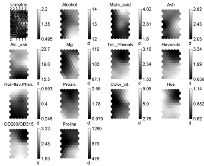
Fig. 6. Self-Organizing Map of the Wine data
