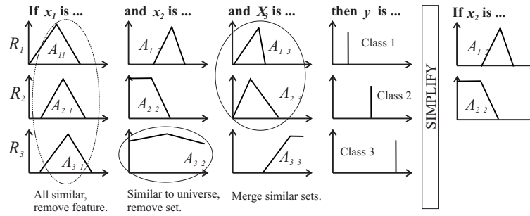
Fig. 2. Similarity-driven simplification.
