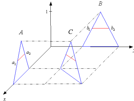
Figure 3: The case of \rho(A, B) = -1 .
