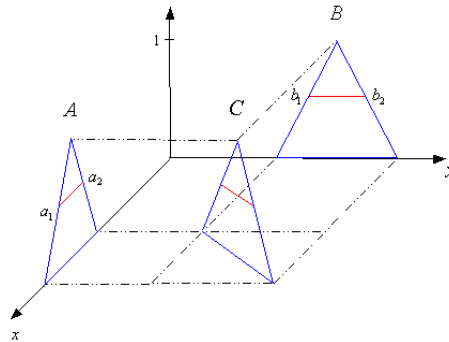
Figure 2: The case of \rho(A, B) = 1 .
