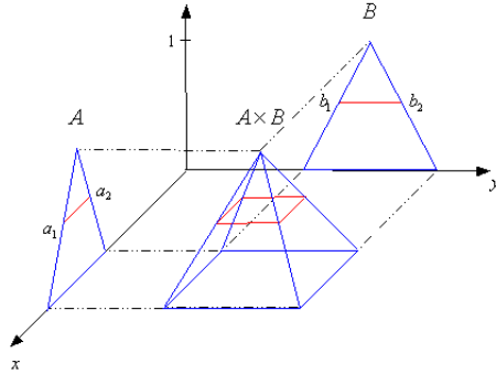
Figure 1: Independent possibility distributions.
