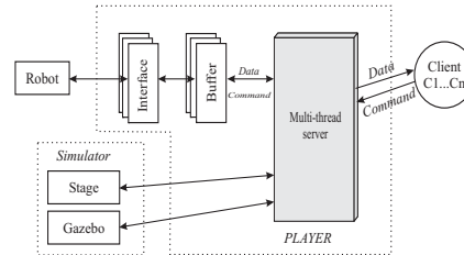
Figure 10 The Player server architecture
