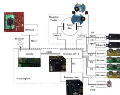
Figure 1 The ZeeRO architecture
