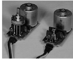
Figure 5 Servomotor with feedback sensor (left) and with resistor array (right)
