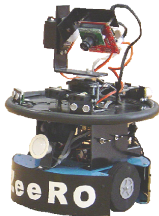
Figure 11 The ZeeRO mobile robot
