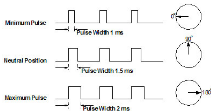
Figure 4 Rotation angle function of the command pulse width
