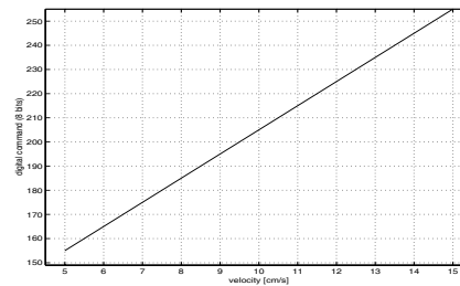
Figure 6 Command signal function of desired linear velocity
